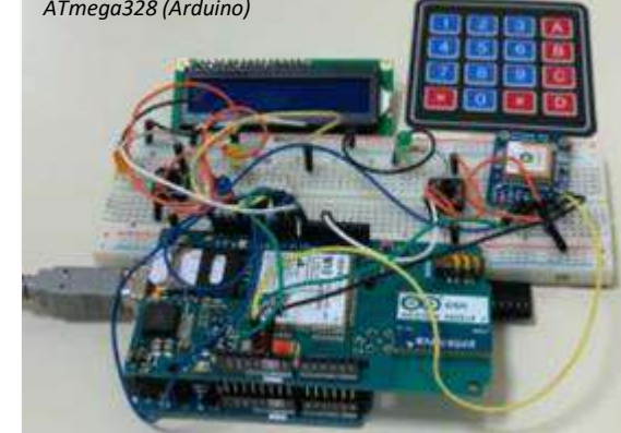
GSM/3G enabled, GPS device based on ATmega328 (Arduino)
