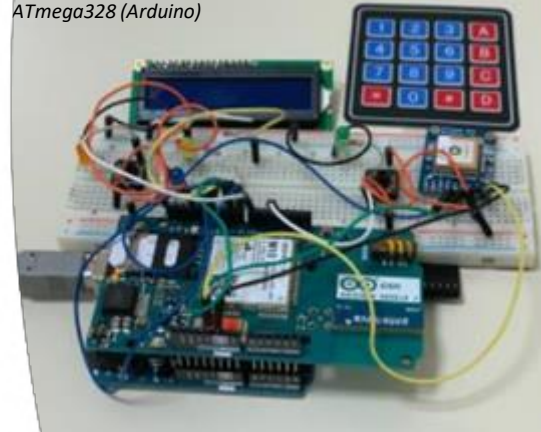
GSM/3G enabled, GPS device based on ATmega328 (Arduino)
